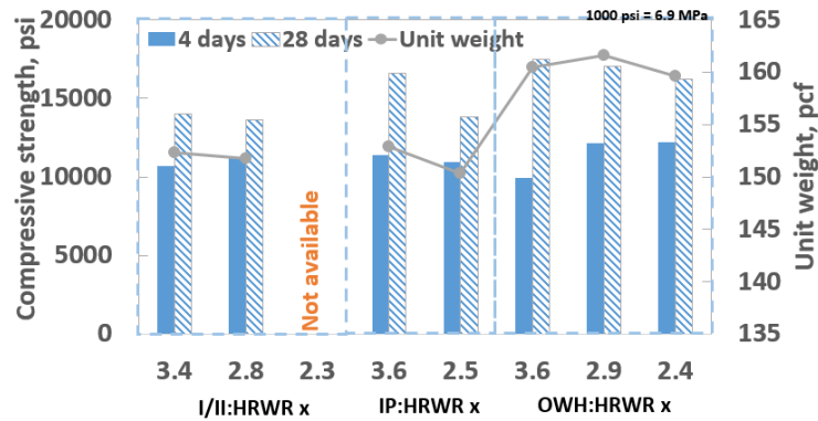
(b) Compressive strength
