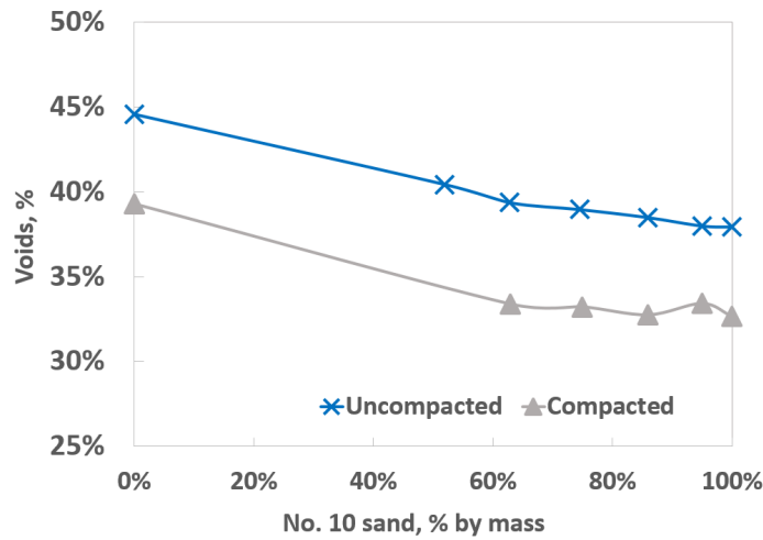
Figure 4.3 Uncompact and compacted void contents of aggregates in No. 10 sand matrix
