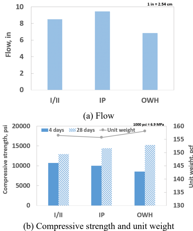
Figure A.1 Impacts of cement type on UHPC performance
