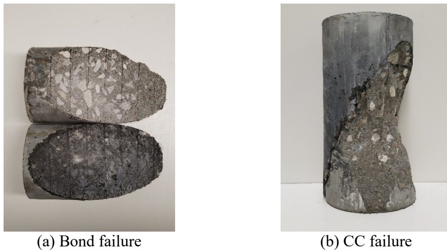
Figure 5.9 Slant shear specimen failure modes
