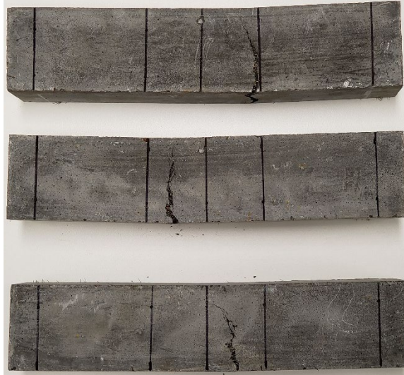
Figure E.3 UHPC 1900-A flexural specimens failure modes
