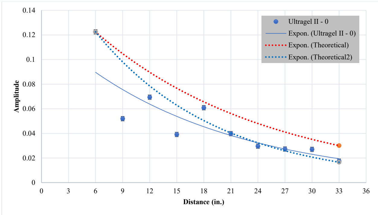
Figure 14. 0-degree Specimen: Ultralag II Results on the 0-degree Specimen
