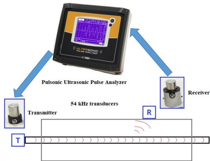
Figure 5. Experimental set-up for UGWL testing procedure
