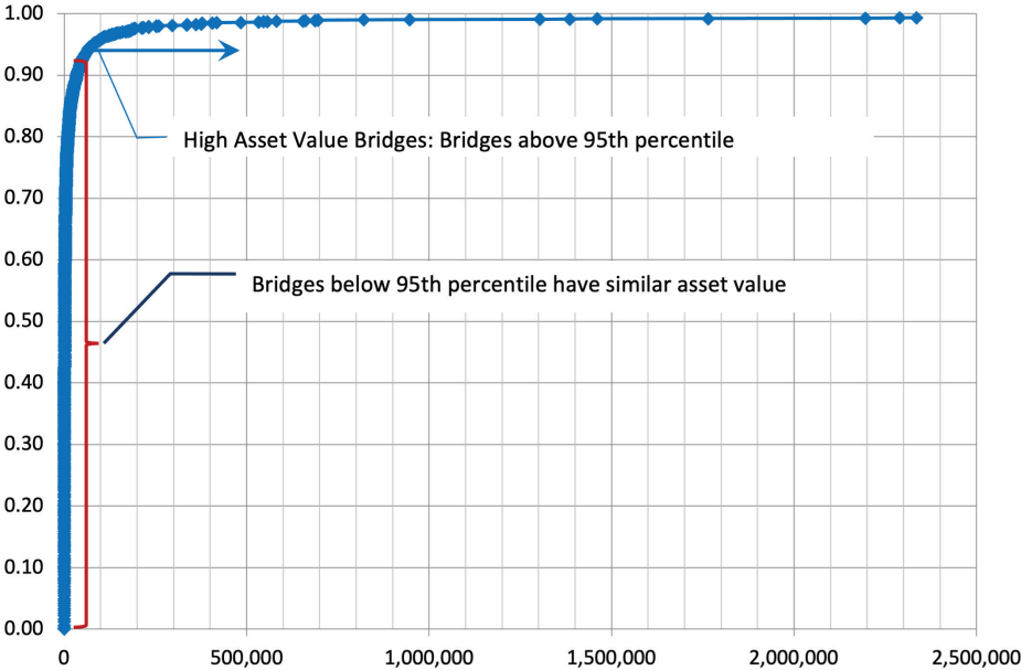
Figure 29 - Cumulative Distribution of Asset Value for State Highway Bridges
