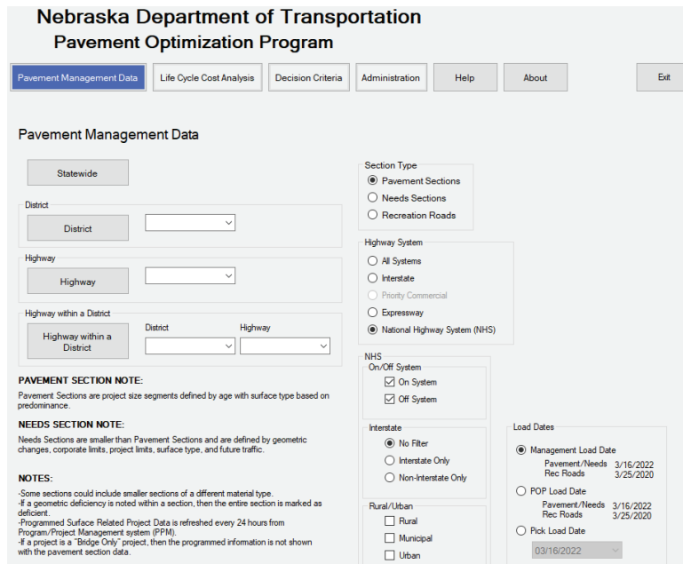
Figure 12 - POP Pavement Management Data Screen
