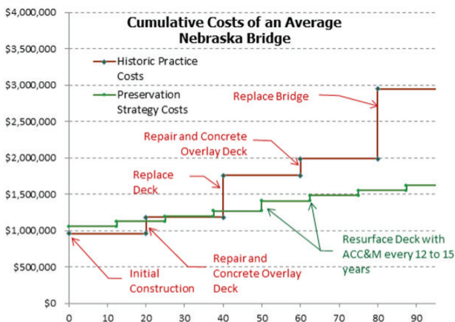
Figure 24 - Cumulative Cost of Average Bridge with Historic and Current Preservation Strategies
