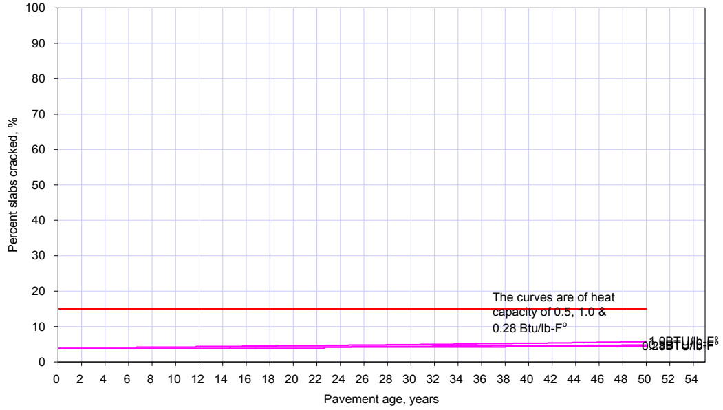
Predicted Cracking
