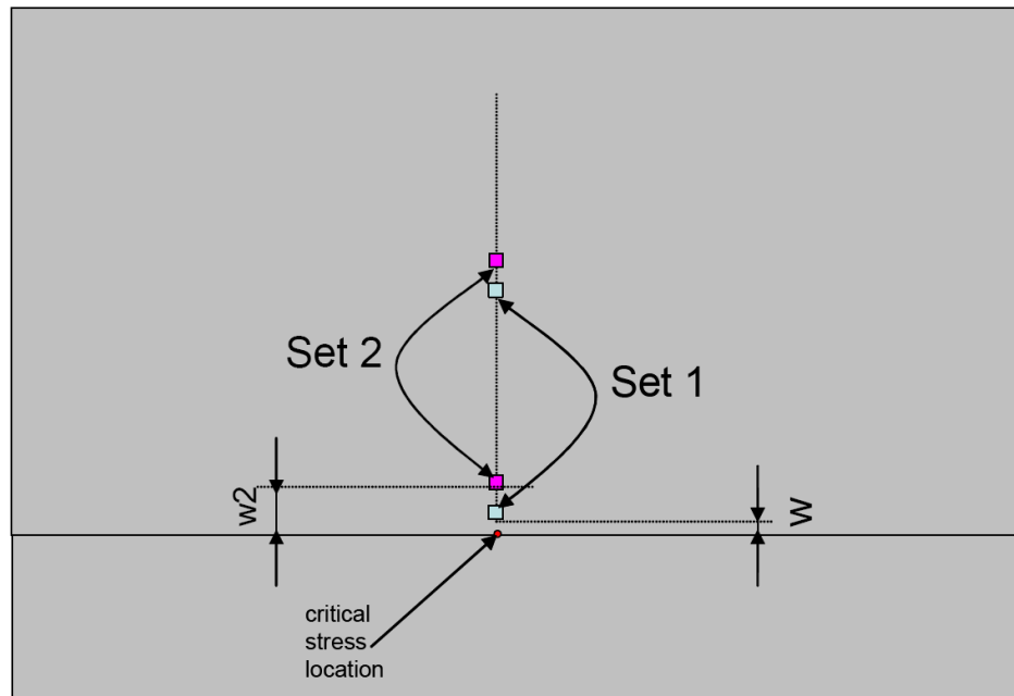
Figure 2-3. Analysis of a single axle load with dual tires using NNB1 (NCHRP 2003; Appendix QQ).
