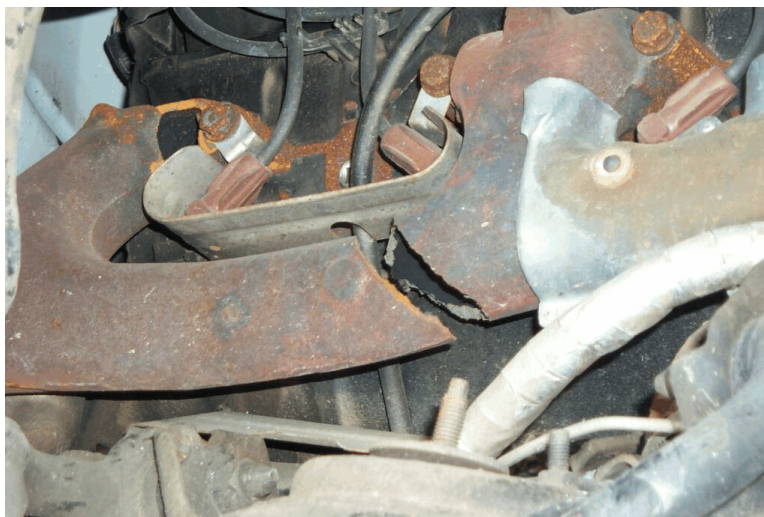
Figure 39. Vehicle Undercarriage Damage, Test NIT-1
