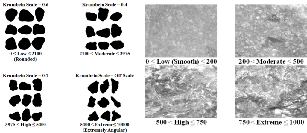
a) Aggregate angularity rankings b) Aggregate texture rankings Figure 6.4. Direct measurement of aggregate shape and texture
