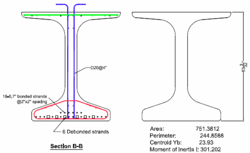
Figure 11: Section properties at the girder ends
