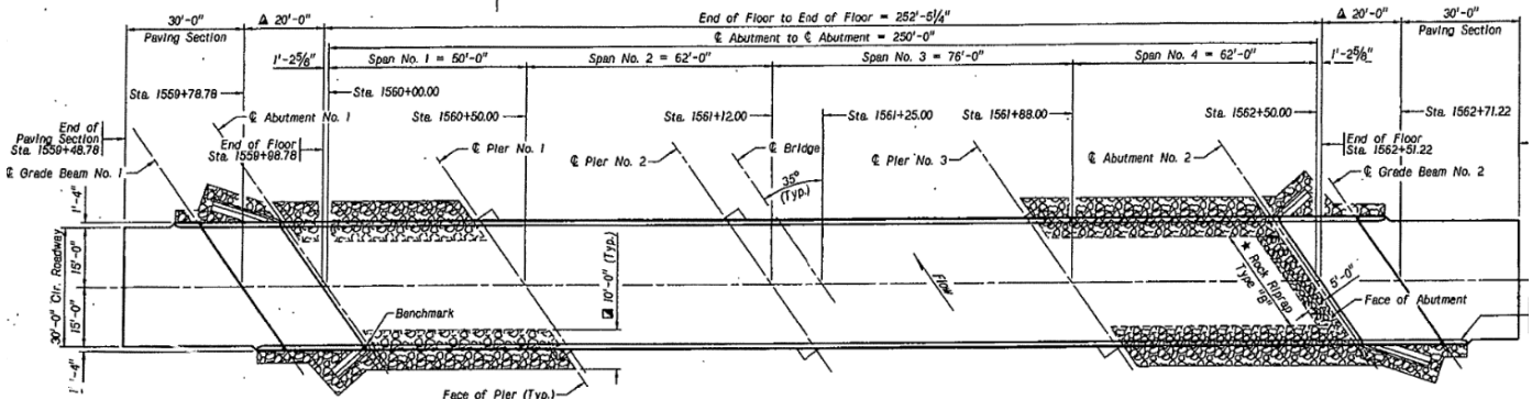
Figure 3.1: Plan view of Ayr Bridge
