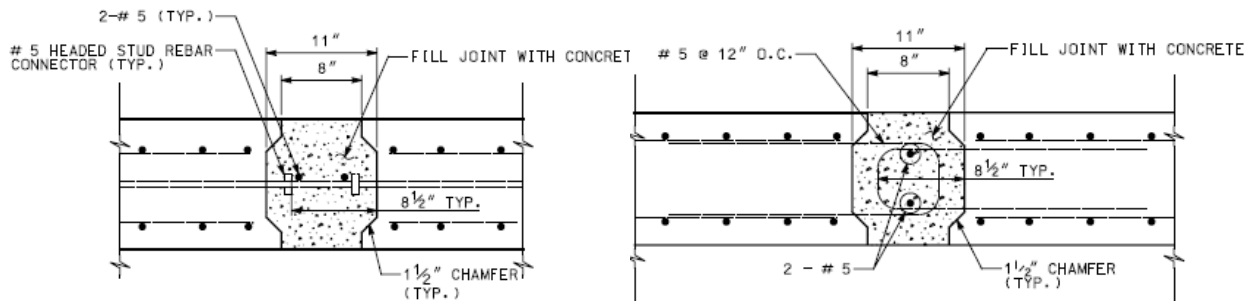
Figure 5.6: Options of longitudinal joints (PCI, 2012)
