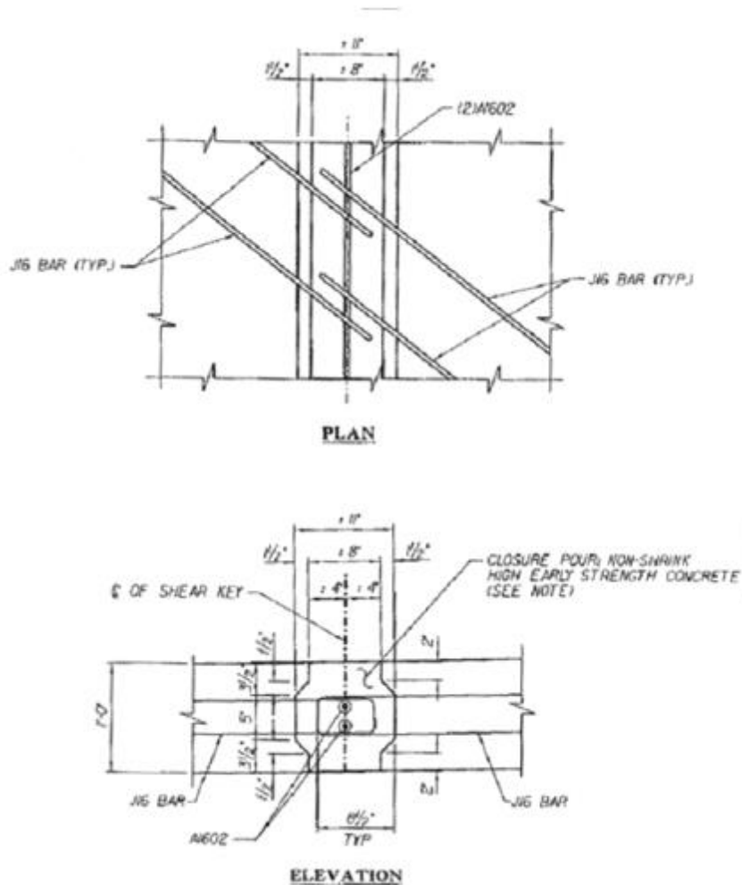
Figure 5.15: Plan and elevation views of longitudinal joint (Ziehl et al., 2015)
