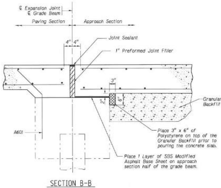
Figure 2.2: NDOT Typical Approach Slab Design and Detailing
