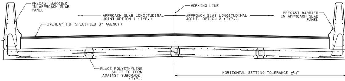
TYPICAL SECTION: SUB-SURFACE APPROACH SLAB WITH INTEGRAL BARRIER
