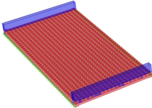
Figure 4.4: Extruded view of the approach slab model
