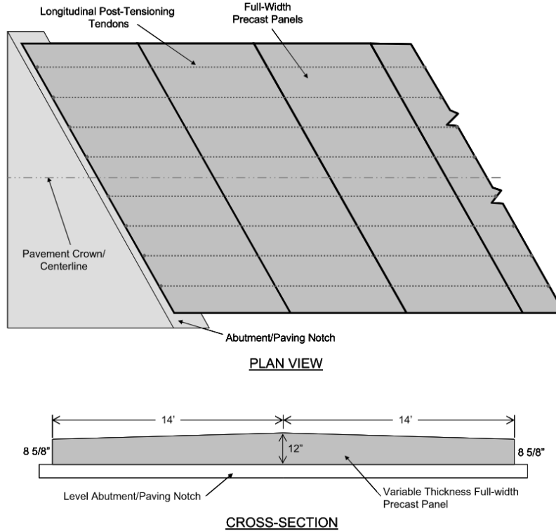
Figure 5.2: Full-Width Precast Concrete Approach Slabs (Merritt et al., 2007)
