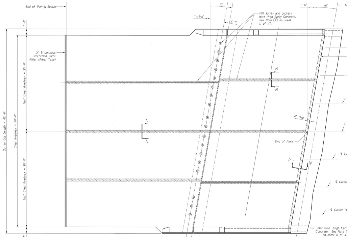
Figure 5.23: Plan view of the precast approach slab and paving section panels (Belden-Laurel Bridge)
