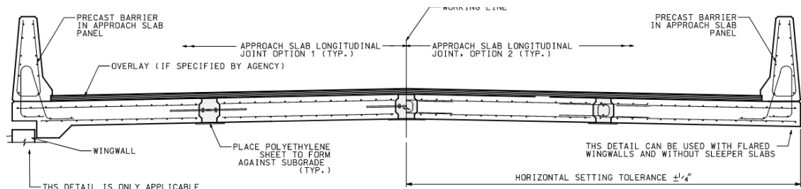
TYPICAL SECTION: SURFACE APPROACH SLAB WITH INTEGRAL BARRIER
