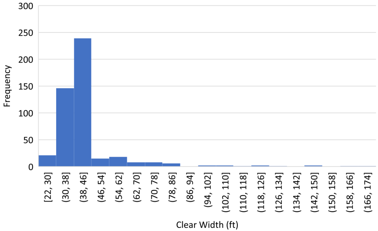
Figure 3.14: Frequency distribution of roadway clean width of the considered NDOT approach slabs
