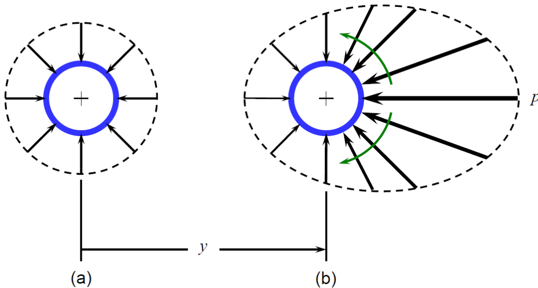
Figure 5.8: Distribution of Stresses around a Pile, (a) Before Lateral Deflection, (b) After Lateral Deflection (retrieved from LPILE 2019 Technical Manual)
