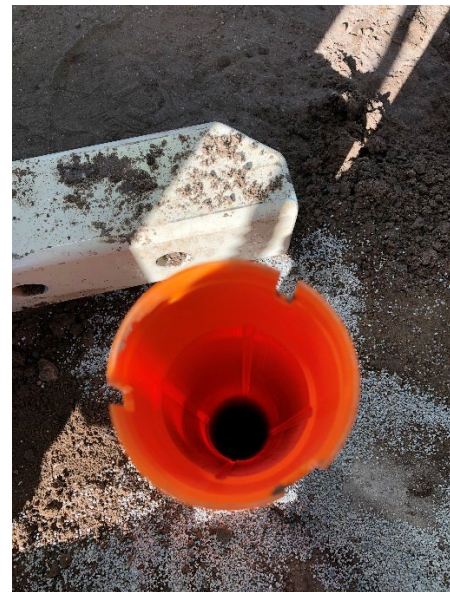
Figure 3.22: Orthogonal Grooves in each Casing (left figure retrieved from Inclinometer Manual)
