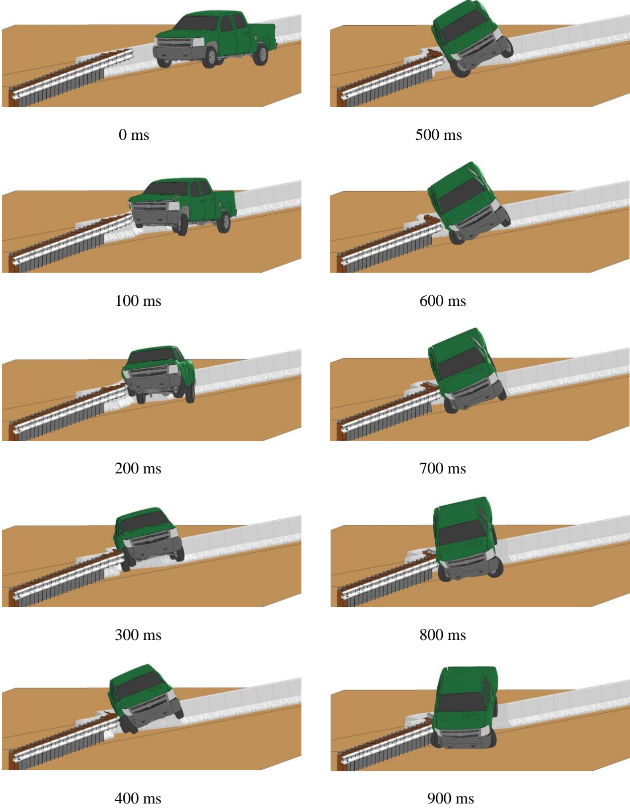
Figure 89. Reverse-Direction Impact Sequentials, Impact Location No. 2
