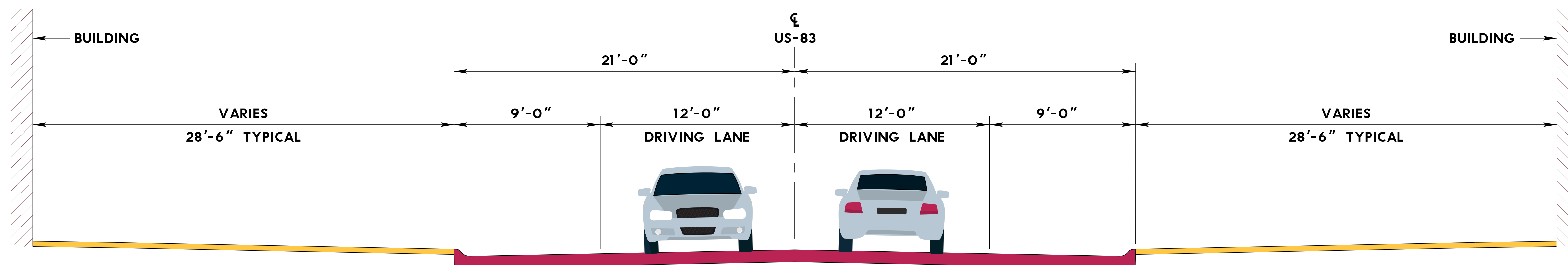
HWY. US-83/MAIN ST. FROM 1ST ST. TO 4TH ST. (AT SIDEWALK BUMP OUT)
