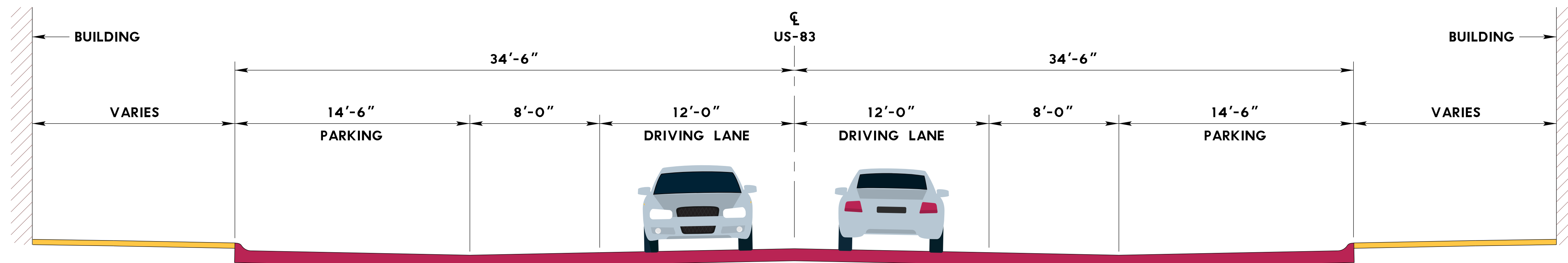
HWY. US-83/N. MAIN ST. FROM 1ST ST. TO 4TH ST. (WITH ON-STREET PARKING)
